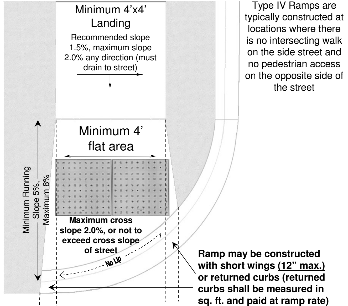
Type IV - (Special Application) Curb Ramp
